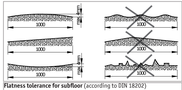
Flatness tolerance for subfloor (according to DIN 18202)
